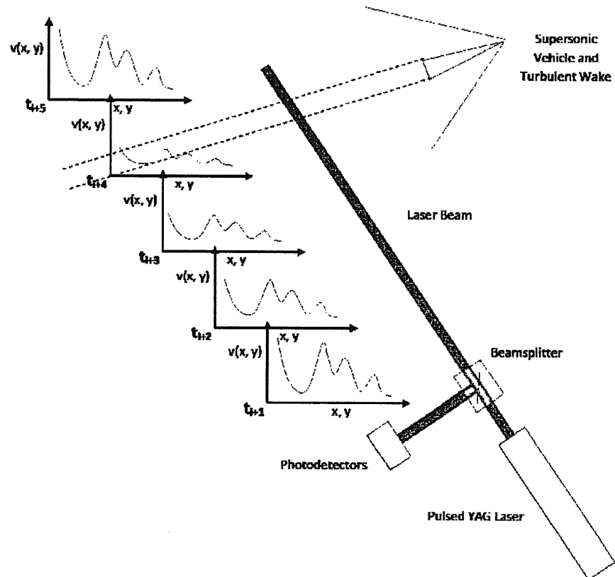
Figure 17. Schematic of a Pulsed LIDAR System.
