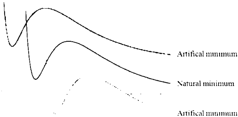
Figure 7. A Combination of Phenomenologically Viable Fields Generates a Stable Minimum of the Vacuum Energy Density at a Fixed Higher Dimensional Radius. This stable minimum, located at a positive energy, indicates a stable deSitter type spacetime and reflects a realistic dark energy model. Note in this plot that the radius of the extra dimensions is shown on the x-axis, and the energy density on the y-axis (normalized units are used).
