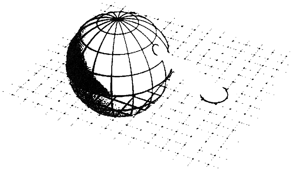
Figure 19. Stereographic Projection
